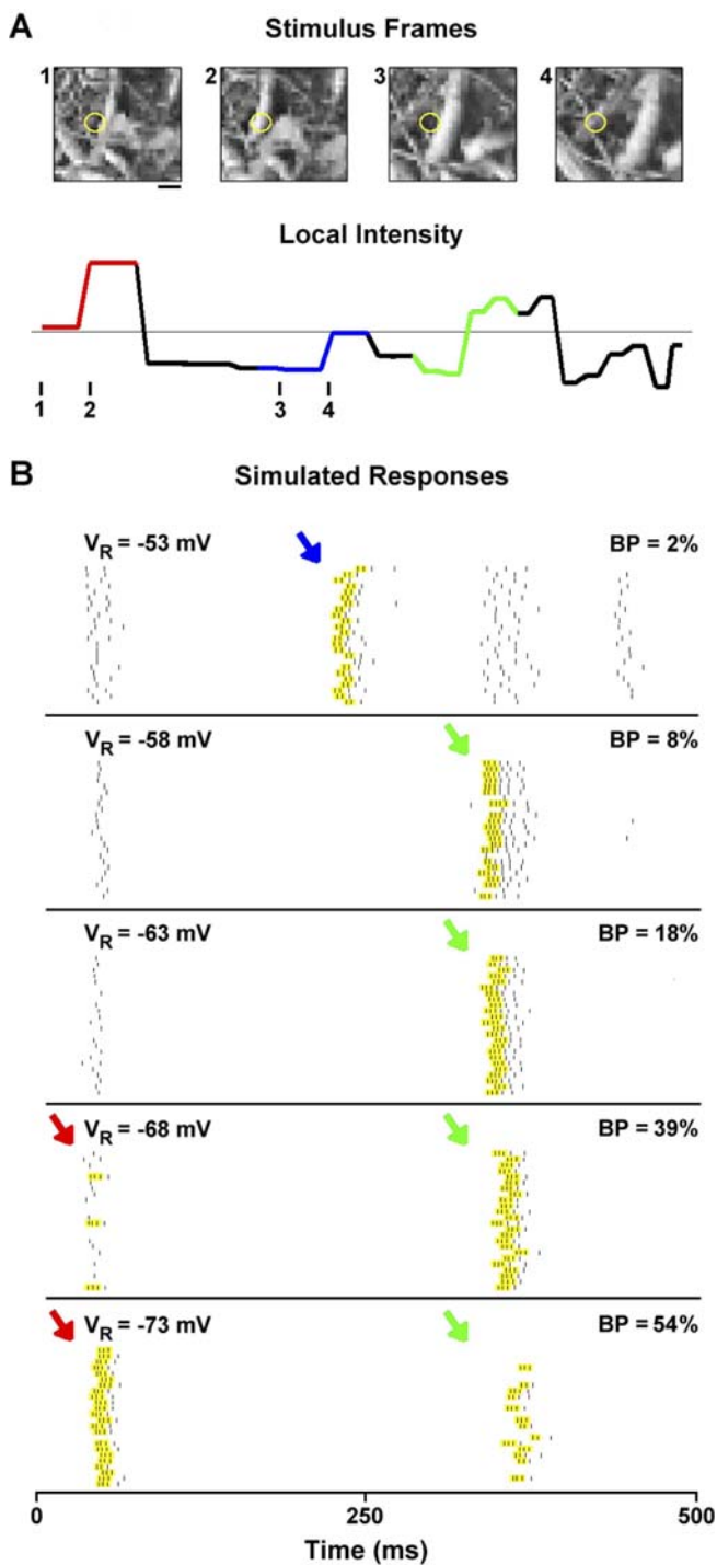
Figure 1. Simulated LGN Responses to Natural Scene Movies at Different Resting Potentials
