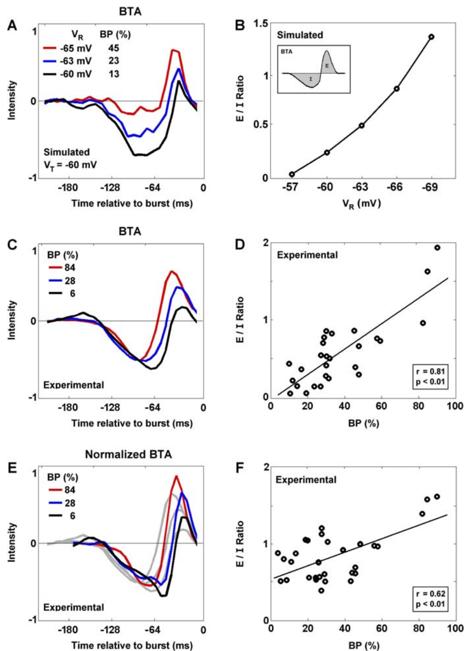
Figure 2. The Luminance Sequences That Trigger Burst Events
