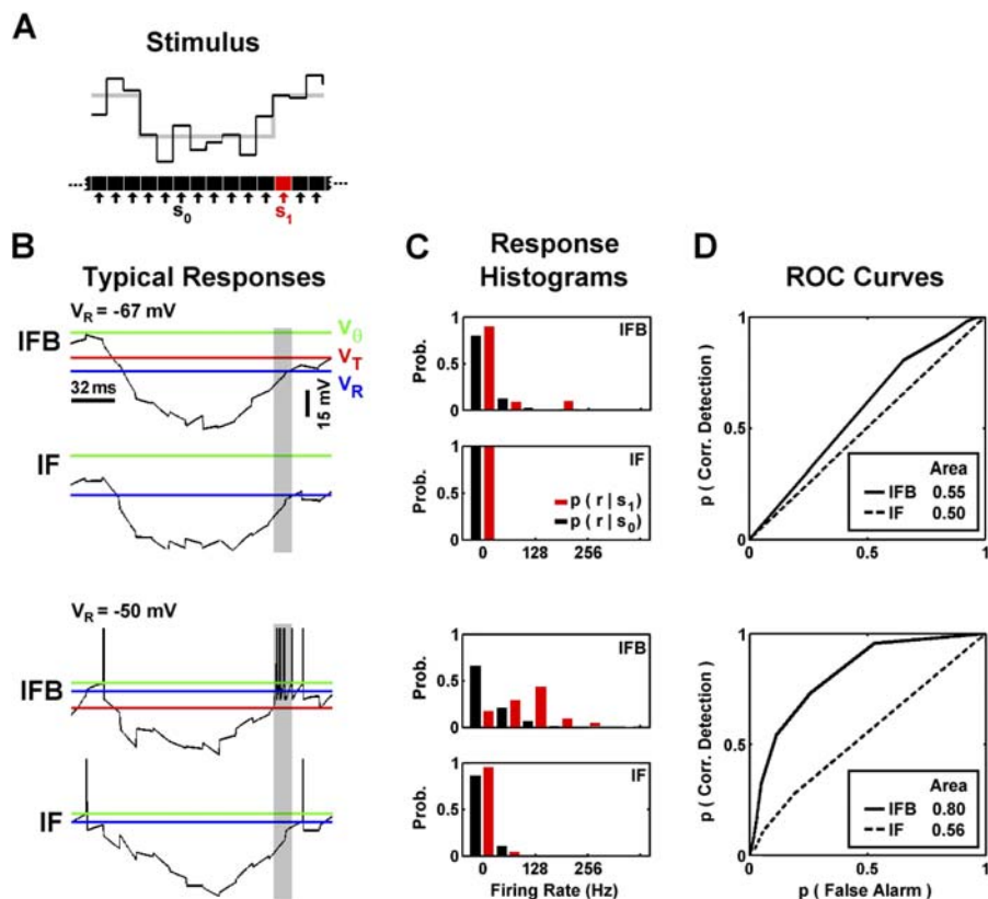
Figure 4. Detection of the Offset of Inhibitory Luminance Sequences
